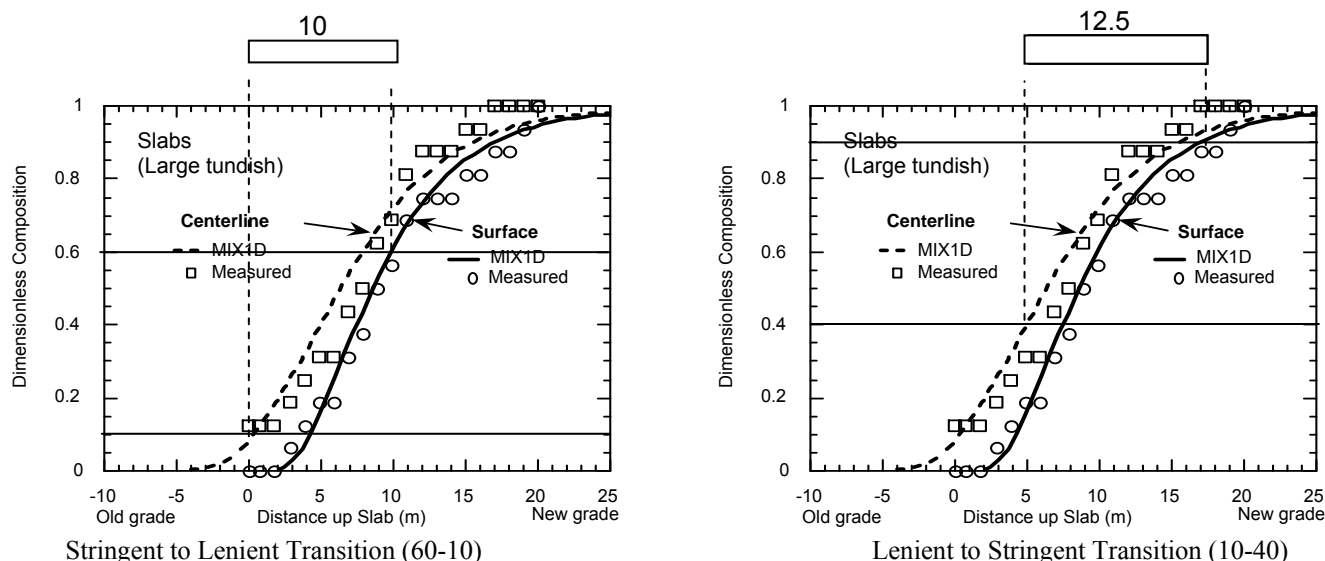
Figure 28. Computed location of slab to downgrade, for the same composition profiles with different grade specifications
