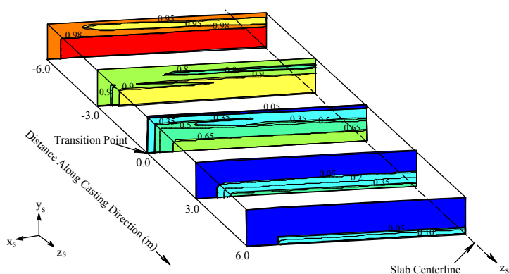
Figure 26. Composition distribution in strand (3-D model)
