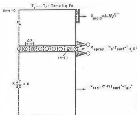
Figure 3. Schematic of continuous cast steel strand, showing 1-D slice domain and boundary conditions 5
