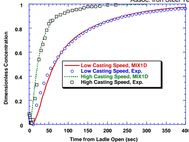
Figure 24. Concentration Evolution from the tundish
