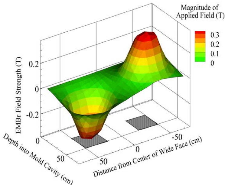
Figure 16. Measured electromagnetic field contours (0.355T)
