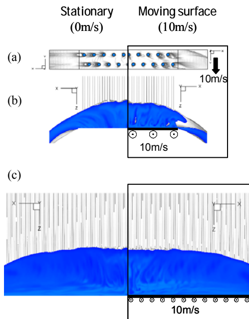
Figure 21. Water pool height comparison between stationary and moving surfaces (a) 300mm width (top view) (b) 300mm width (front view) (c) 1,200mm width
