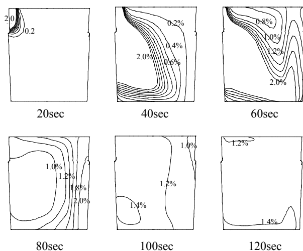
Figure 6. Mixing concentration predicted in centerplane (time after start of ferroalloy addition) 17
