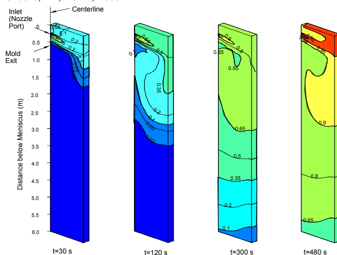
Figure 25. Concentration evolution in the strand
