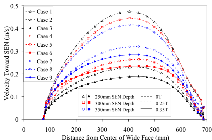
Figure 18. Velocity across top surface toward SEN for Table 2 cases
