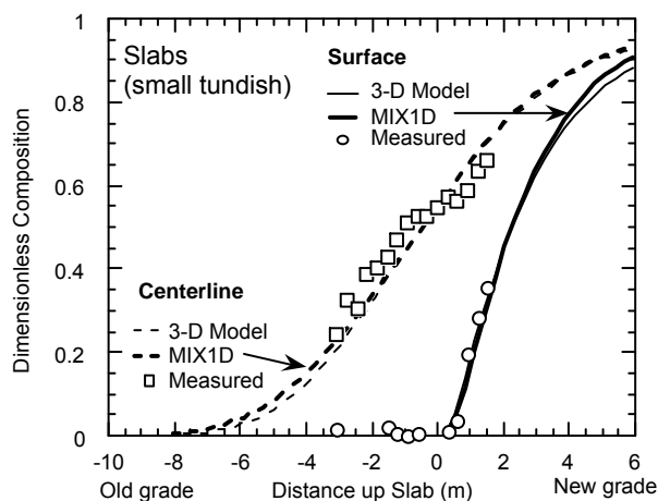
Figure 27. Composition distribution in strand
