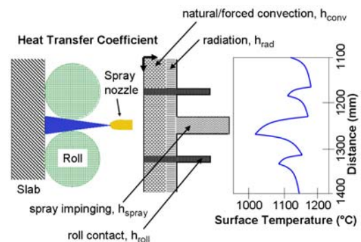
Figure 31. Schematic of spray zone region, heat transfer coefficients, and corresponding surface temperature variations
