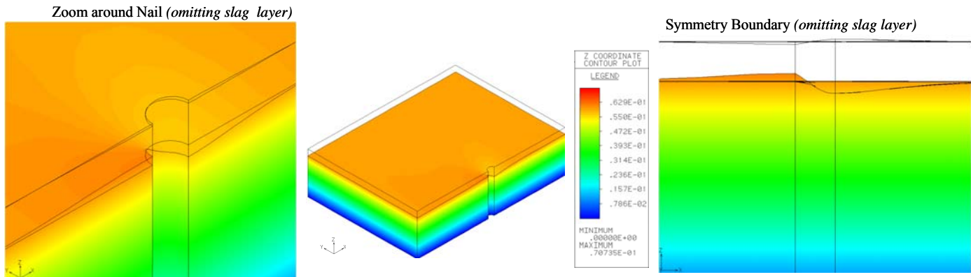
Figure 13. Model of slag / steel interface shape and vertical (z) velocity contours: 3 views (0.3 m/s; 10-mm diameter nail)
