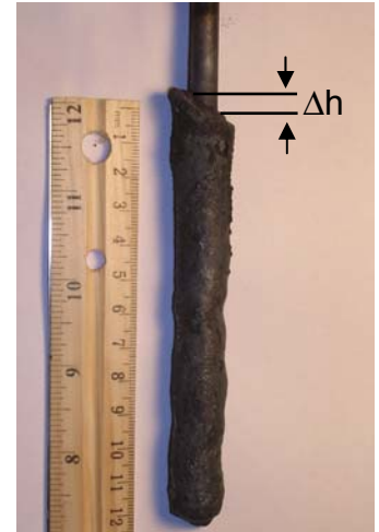
Figure 12. Nail photo showing measurement of solidified knob
