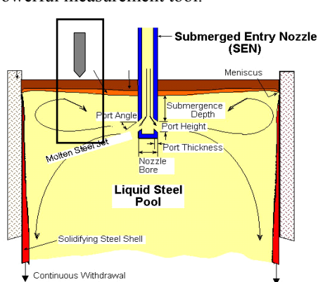
Figure 8. Continuous casting mold showing steel flow, top surface slag layers, and location of nail-board insertion 1)
