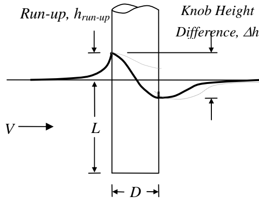
Figure 11. Schematic of flow variables: run-up height and measured knob height difference
