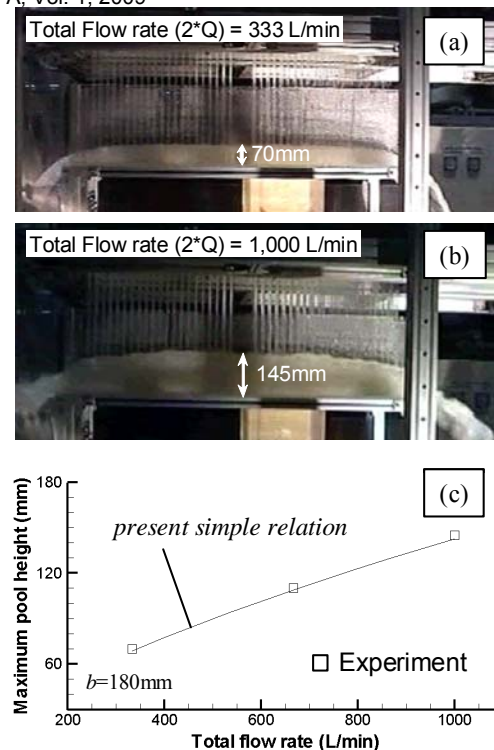
Figure 22. Comparison of water pool height
