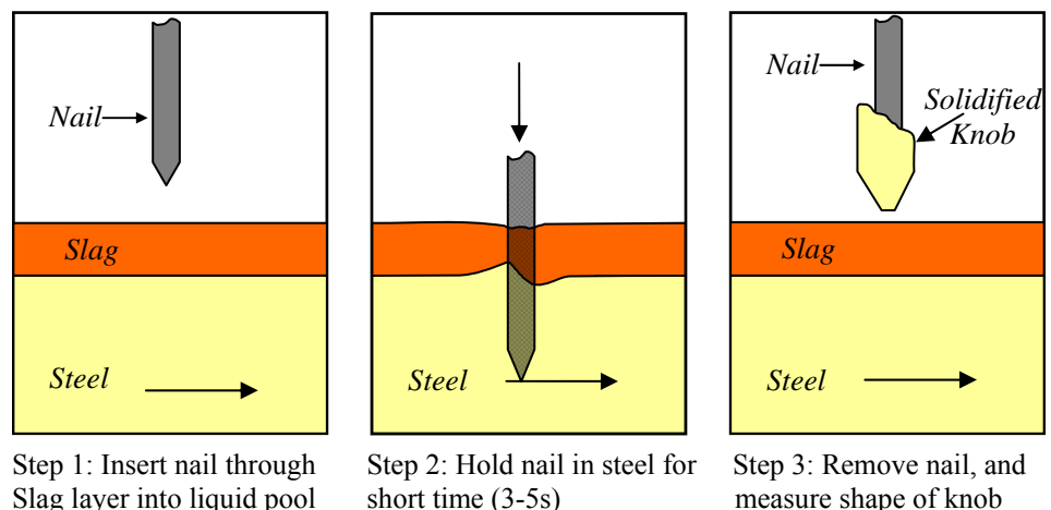
Figure 9. Nailboard method to measure steel surface speed and direction
