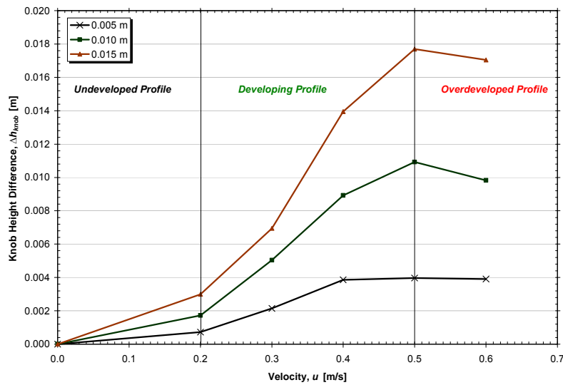
Figure 14. Relation between steel surface velocity and measured height of knob from nail-board test (with slag)
