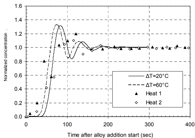
Figure 7. Computed concentration profiles at the sampling point compared with plant measurements 17
