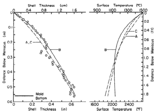
Figure 4. Liquid pool and surface temperature profiles in the mold, comparing finite difference model (A) with analytical solution (C), and finite difference model (B) with shell thickness measured near a beam blank web 6
