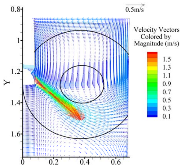
Figure 17. Velocity vectors on the mold wide face centerplane for Case 6: outer circle shows extent of EMBR field, and inner circle showing region of strongest field.
