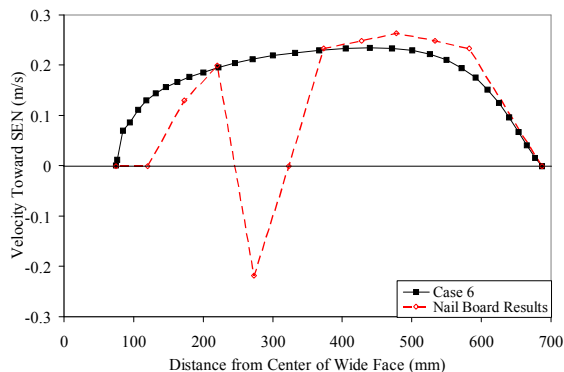
Figure 19. Comparison of calculated and experimental meniscus velocity
