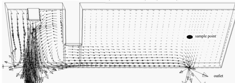
Figure 23 a). Isothermal flow pattern (or high-carbon steel pouring into low-carbon steel)
