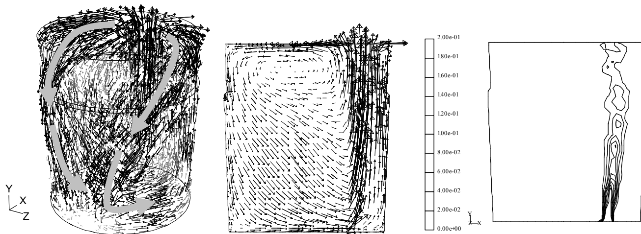
Figure 5. Calculated time-averaged flow field and bubble distribution 17
