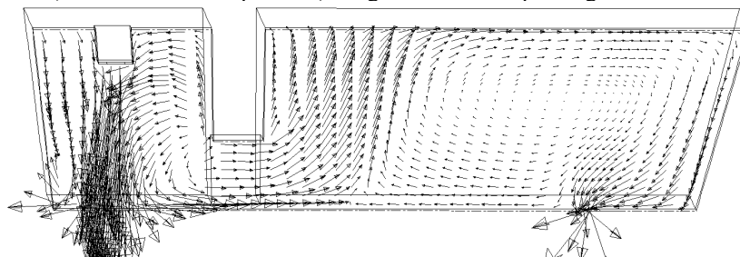
Figure 23 b). Flow pattern for hot new steel flowing into a full tundish of 5°C cooler steel (or low-carbon steel pouring into high-carbon steel)
