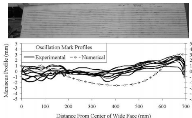
Figure 20. Comparison of calculated meniscus profile with oscillation marks (Case 6)
