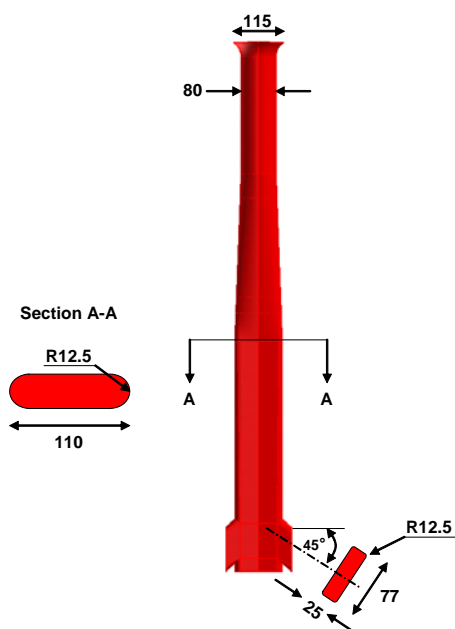
Figure 15. Nozzle Geometry
