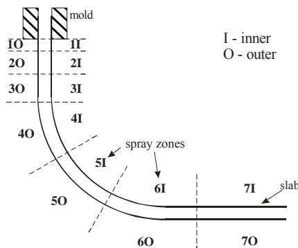
Figure 30. Simulation zones of the model domain from mold to cutoff shear.
