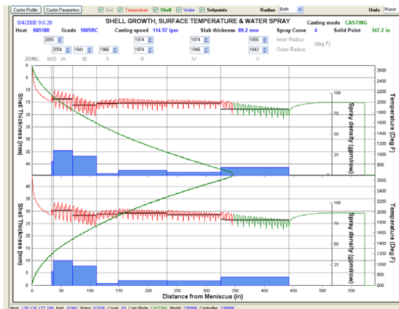
Figure 32. Real-time monitor interface, displaying shell thickness profile, surface temperatures, setpoints, flow rates, etc.
